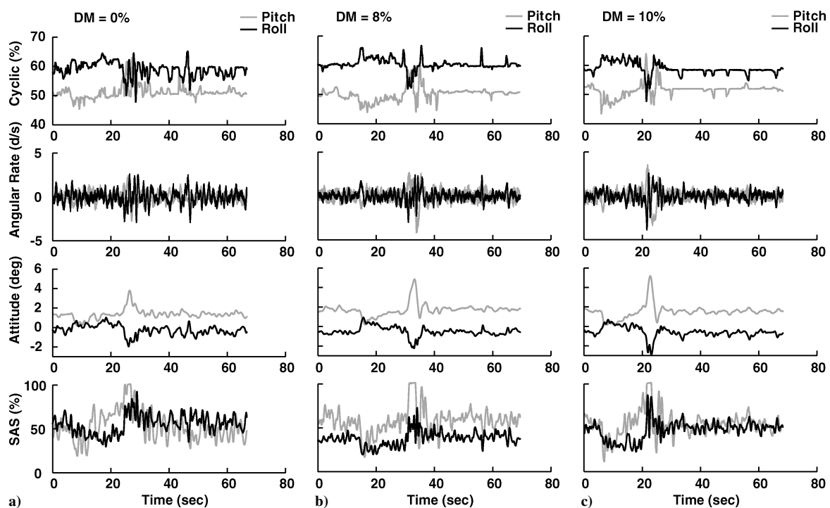
Fig. 20 Comparison of MCLAWS-2 optimized for varying DMs for ADS-33 hover maneuver: a) 0% DM, b) 8% DM, and c) 10% DM.
