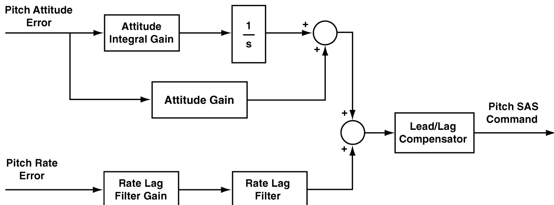
Fig. 12 Simplified schematic of pitch feedback loop.
