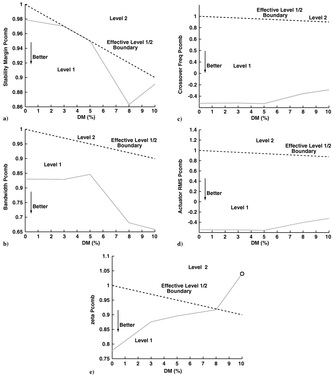
Fig. 15 DM optimization: a) stability margin, b) bandwidth, c) crossover frequency, d) actuator rms, and e) damping ratio.
