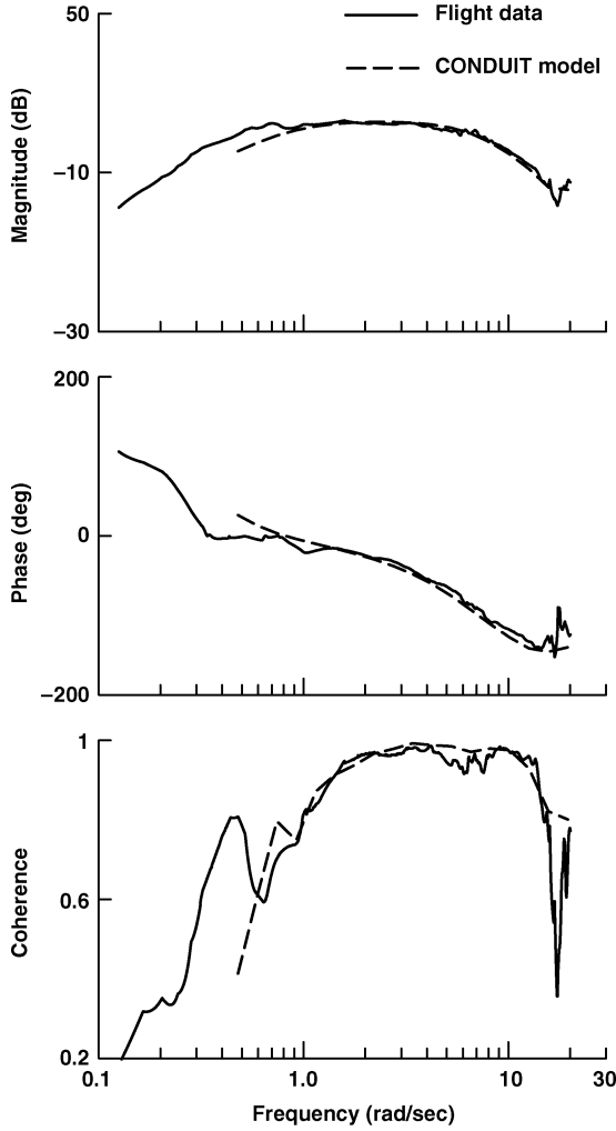
Fig. 8 Unaugmented roll response comparison, p/\delta_{lat_m} .
