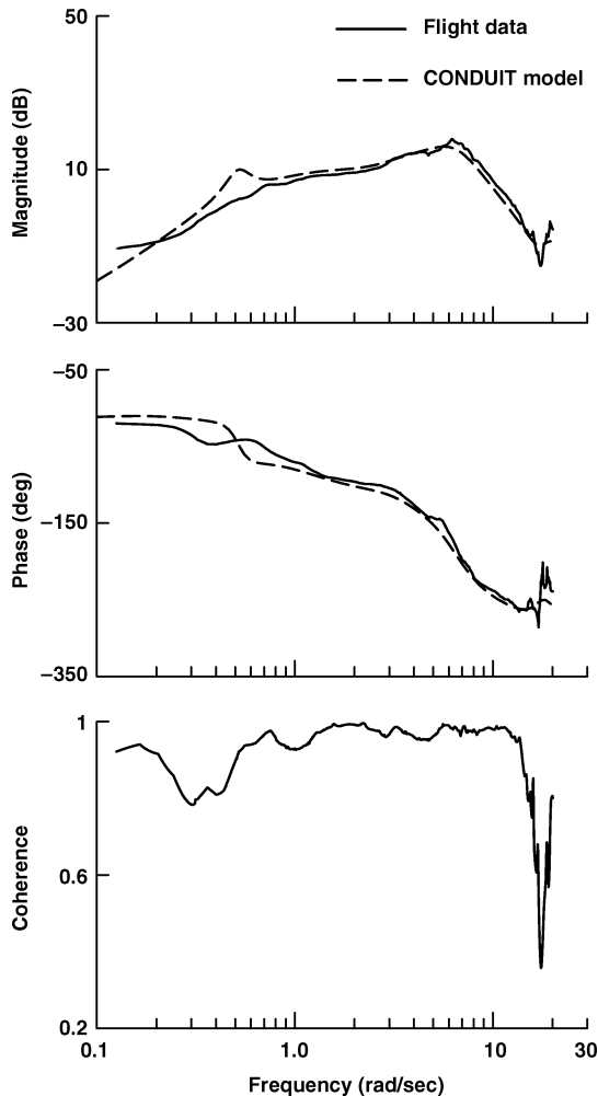
Fig. 10 Roll closed-loop response comparison, p/\delta_{lat} .
