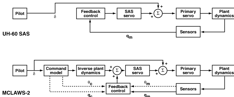
Fig. 1 Standard UH-60 and MCLAWS schematic diagrams.
