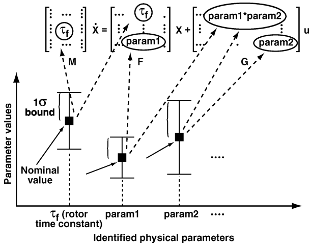
Fig. 17 Example of how CIFER identified physical parameters relate to aircraft state-space model.
