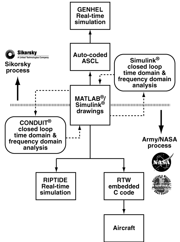
Fig. 2 Pictures-to-code process.
