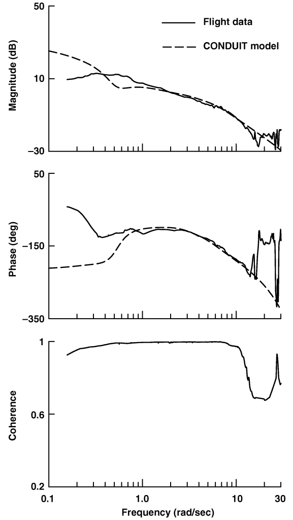
Fig. 9 Roll broken-loop response comparison, Eq. (4).
