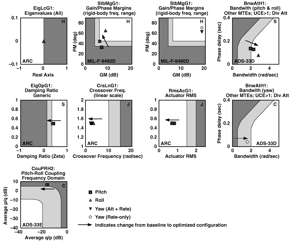
Fig. 11 CONDUIT HQ evaluation for the baseline and optimized baseline (DM=0%) configurations.
