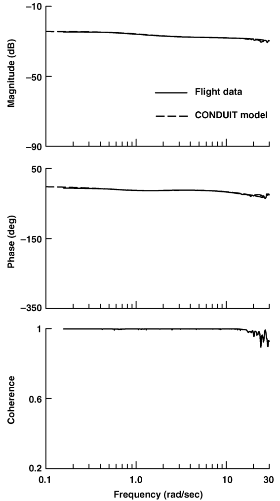
Fig. 7 Roll rate SAS compensation comparison, P_{sas} .
