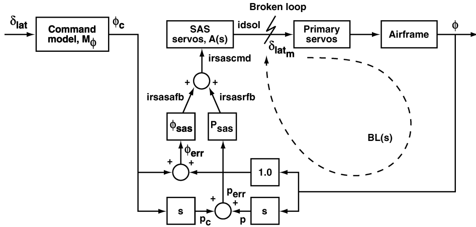
Fig. 5 Simplified schematic of roll axis MCLAWS-2 implementation; measured parameters indicated next to signal arrows.
