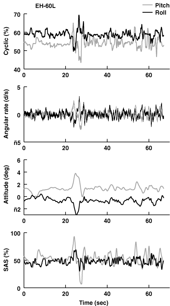
Fig. 19 Time history of EH-60L BLACK HAWK SAS/FPS standard control laws for the ADS-33 hover maneuver.
