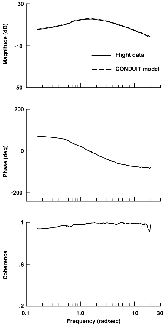
Fig. 6 Command model comparison [sM_\phi(s)] , roll axis.
