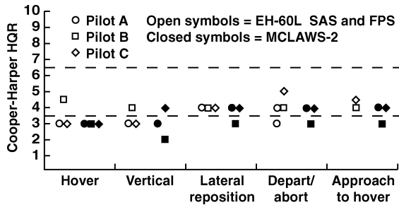
Fig. 21 HQ evaluations of MCLAWS-2 and EH-60L standard SAS/FPS.
